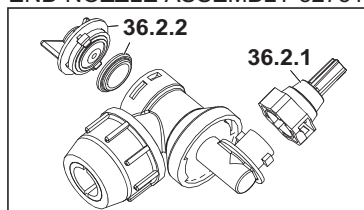
END NOZZLE ASSEMBLY 5275122
