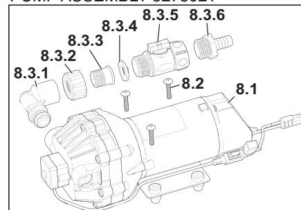
PUMP ASSEMBLY 5278021
