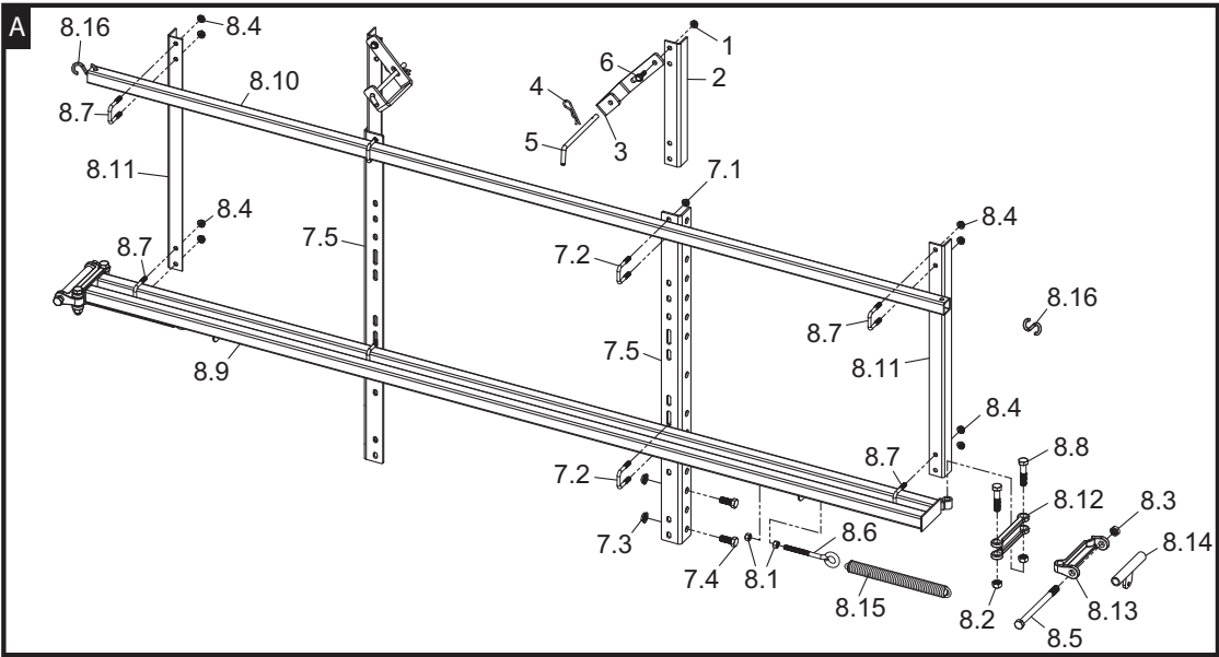
5277359 - 257 BOOM CENTER SECTION ASSEMBLY
