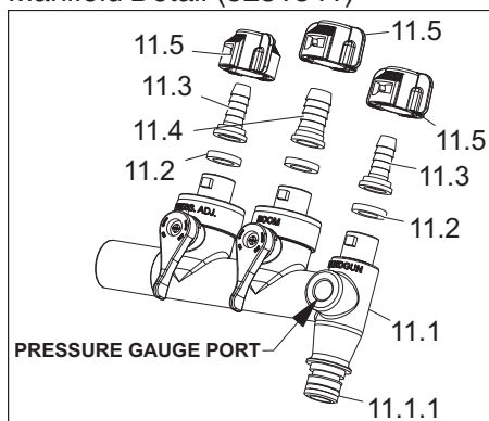
Manifold Detail (5281541)
