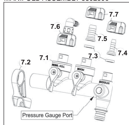
MANIFOLD ASSEMBLY 5302506
