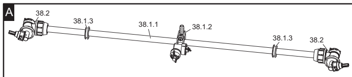
5275260 - WET BOOM ASSEMBLY
