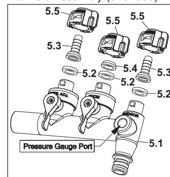
Manifold Assembly (5281536)
