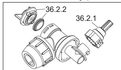
End Nozzle Assembly (5275122)
