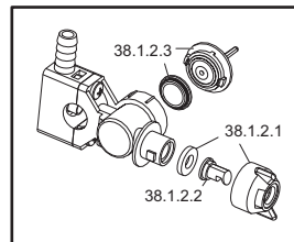
CENTER NOZZLE ASSEMBLY 5275123
