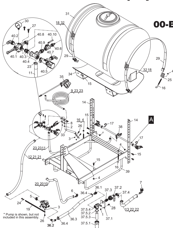
5275260 - WET BOOM ASSEMBLY
