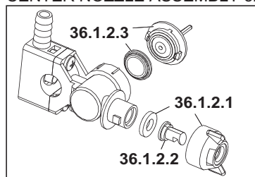
CENTER NOZZLE ASSEMBLY 5275123
