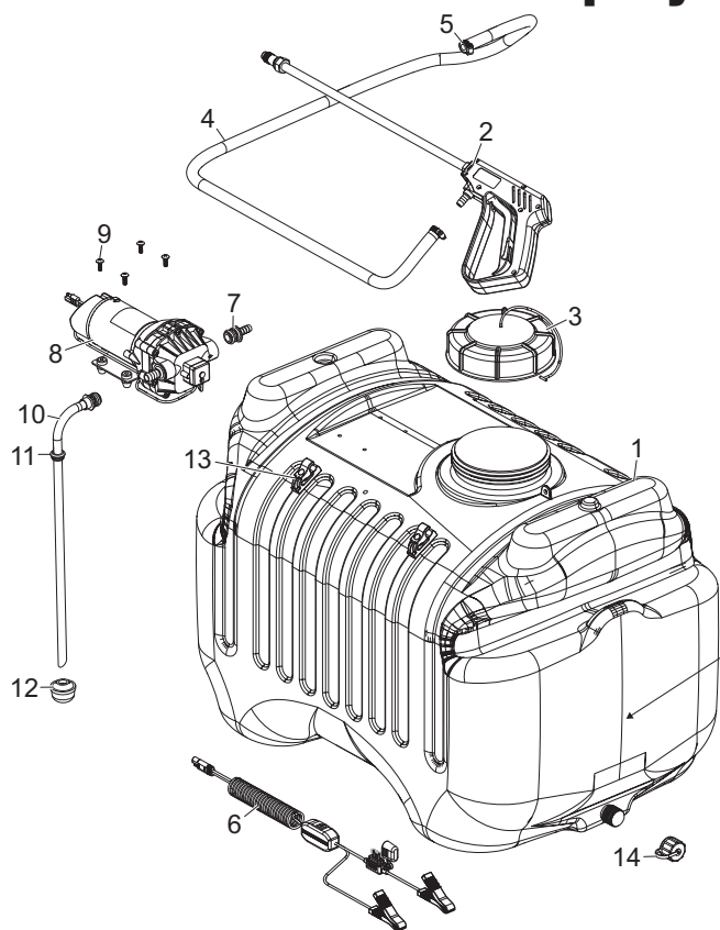
PREVIOUS MODEL (SIDE MOUNTED)
