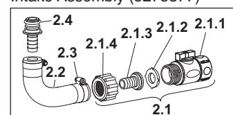
Intake Assembly (5275877)
