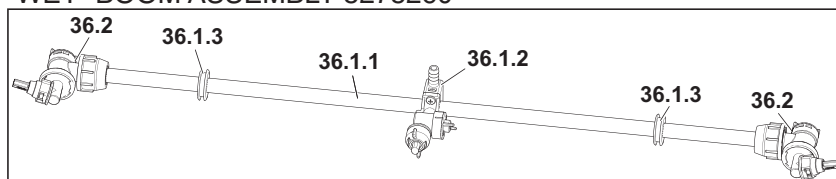
"WET" BOOM ASSEMBLY 5275260
